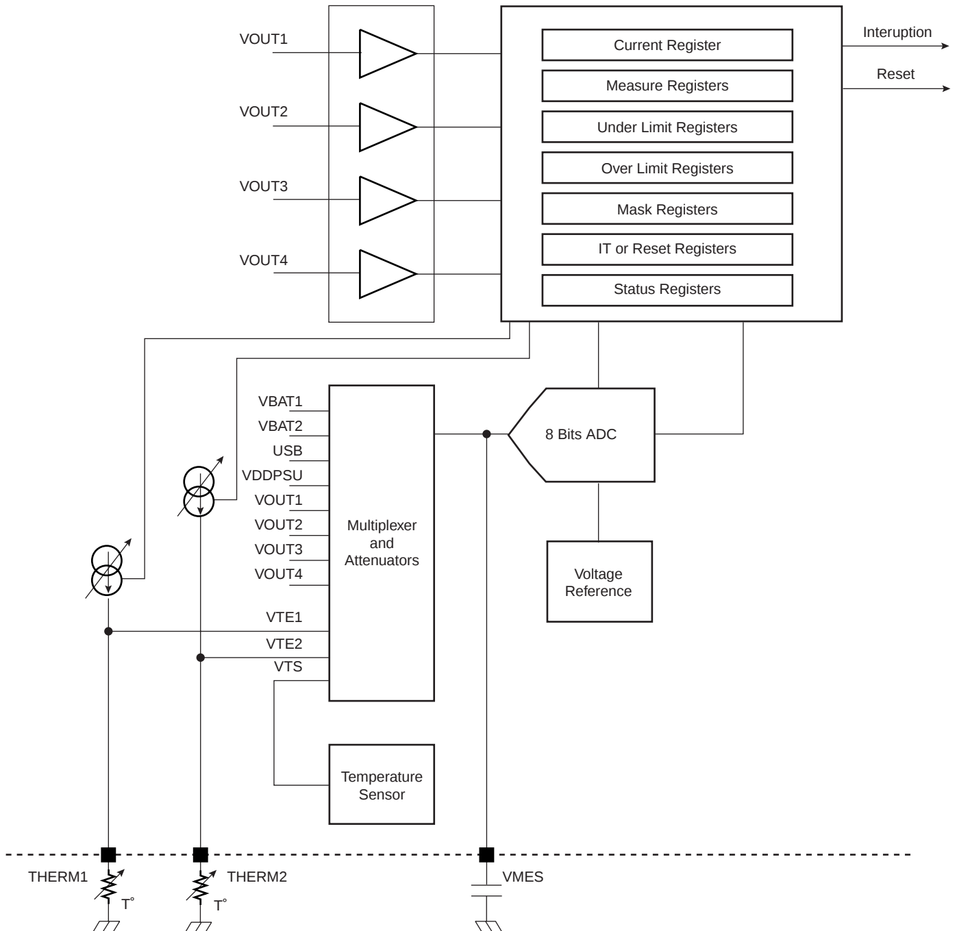
Figure 22. Voltage and Temperature Monitoring Architecture
